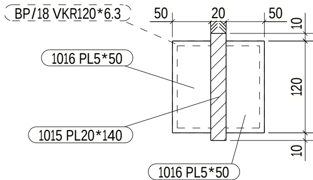
A - A 1:5
